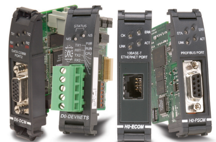
Modbus DeviceNet Ethernet PROFIBUS (Modbus TCP)
