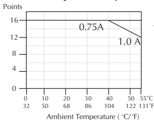
Derating chart for DC outputs
