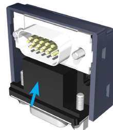
DL06 15-pin high density D-sub port adapter DO-06ADPTR
