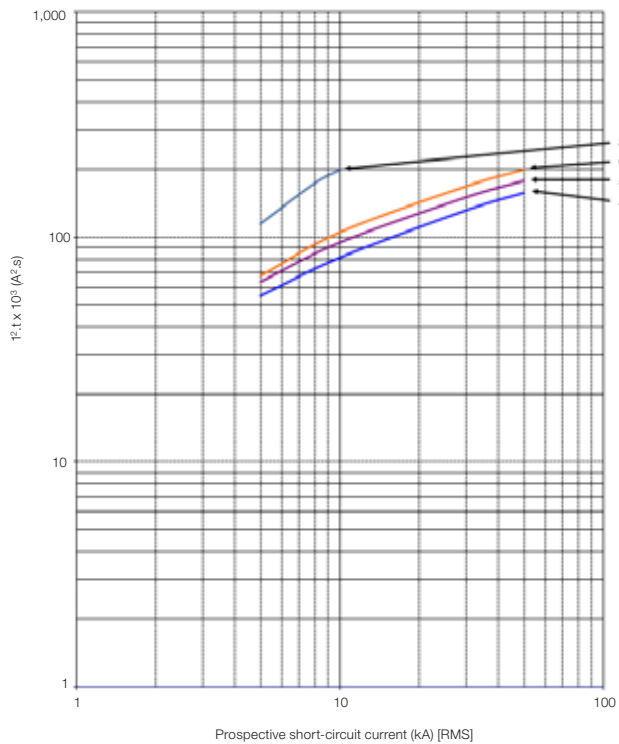
I²t at 415 V - MPW80
