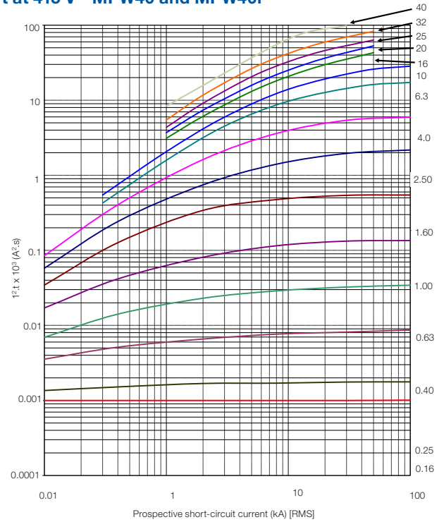
I²t at 415 V - MPW40 and MPW40i
